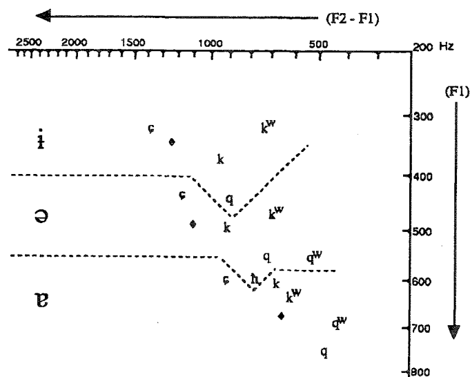
Figure 3. Choi's 1991 spectral analysis of Kabardian vowel allophones. The characters represent the average spectrum of pooled tokens in the respective environments: 'ç' postalveolars, 'k' unrounded velars, 'kw' rounded velars, 'q' unrounded uvulars, 'qw' rounded uvulars, 'h' pharyngeals, '♦' the default allophones.
