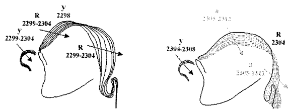
Figure 2. Subject SweB. Frame by frame tongue body movement (13.3ms for each step) in the transition from [y] to [R] (left) and [R] to [a] (right). The numbers refer to frames on the film.
