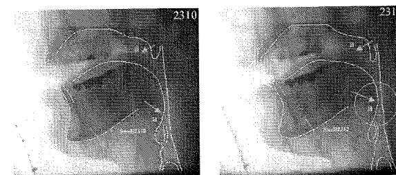
Figure 5. Profiles from the sequence [y:ra], continued from Figure 4. The transition from [R] to [a] continued through frame 2310 (left) to frame 2312 (right), concluding with a narrow low pharyngeal constriction (circled), as expected from Wood (1979).
