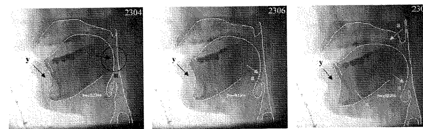
Figure 4. Profiles from the sequence [y:ra], continued from Figure 3. The transition to [R] continued to frame 2304 (left), concluding with a narrow pharyngeal constriction (circled). This retraction was accompanied by slight depression, so that the tongue dorsum passed below the uvula and was directed into the upper pharynx. The lip rounding of /y:/ is still being withdrawn. Activity for /a/ was then commenced, continuing through frames 2306, centre, and 2308, right. The tongue body gesture of /a/ is directed towards the lower pharynx, accompanied by mandibular depression. The velar port opened slightly in frame 2308 (right) (this sequence is phrase final and was followed by a breathing pause). Continued in Figure 5.
